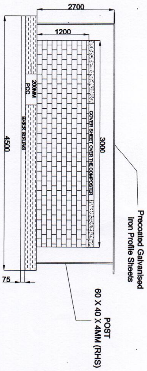
FRONT ELEVATION
